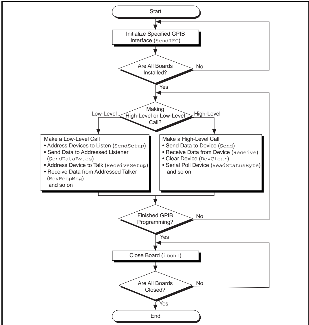
Figure 2-2. General Program Shell Using NI-488.2 Routines
