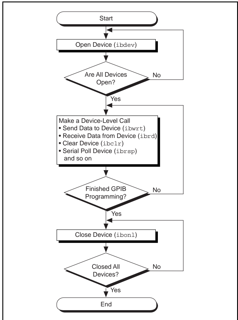
Figure 2-1. General Program Shell Using NI-488 Device Functions
