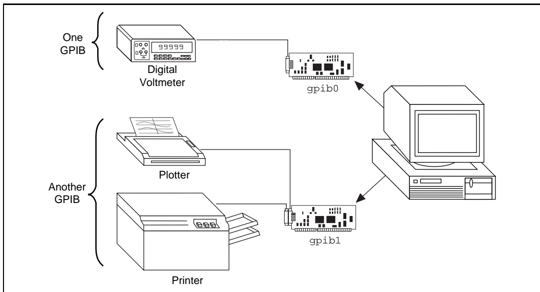
Figure 1-2. Example of Multiboard System Setup
